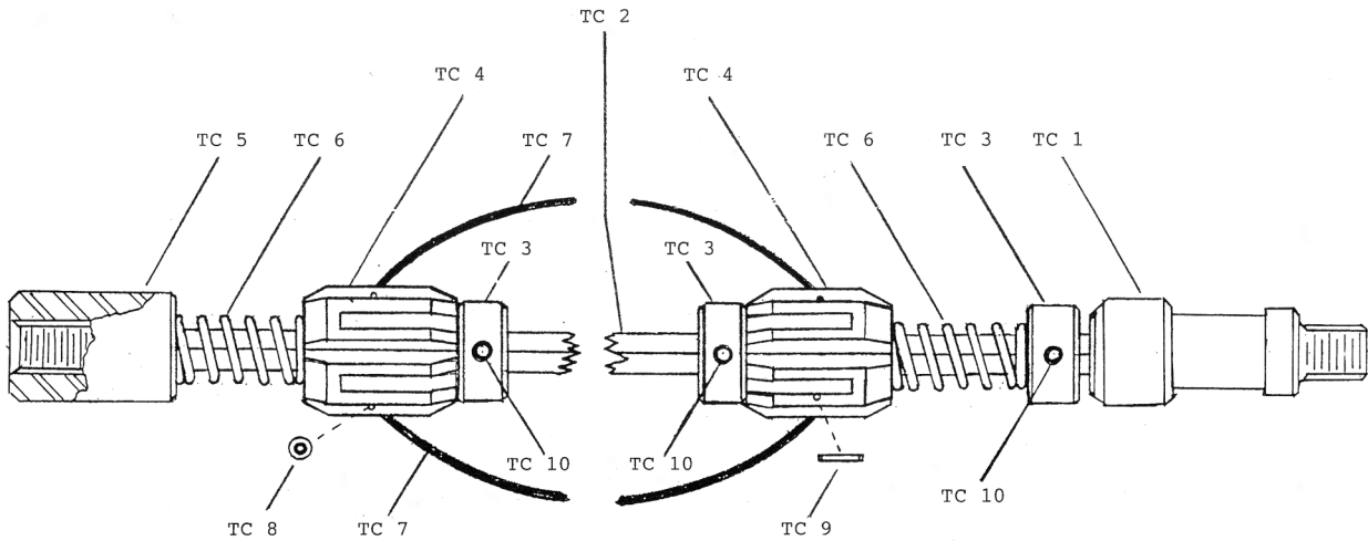
TC 102 Centralizer 9/92
